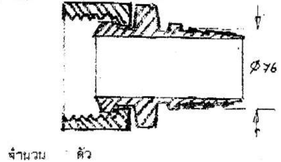
6) GBS-4848 (3" - 11 THREAD SIZE)
