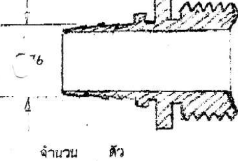
5) CBM-4848 (3" - 11 THREAD SIZE)
