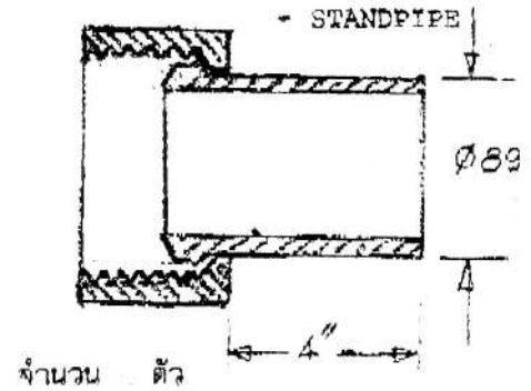
4) 3" BSPT FEMALE SWIVEL LOCK NUT - STANDPIPE
