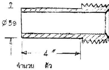
1) 2" BSPT MALE - STANDPIPE
