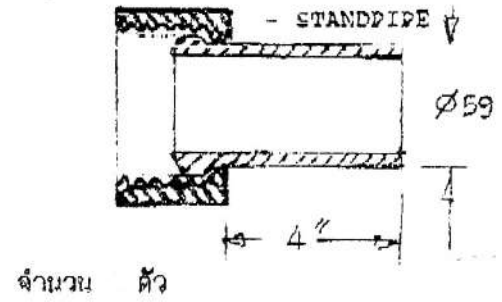
2) 2" BSPT FEMALE SWIVEL LOCK NUT - STANDPIPE
