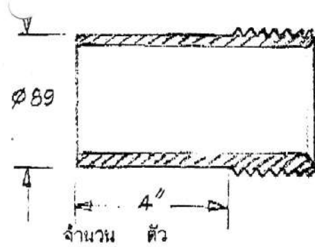
3) 3" BSPT MALE - STANDPIPE
